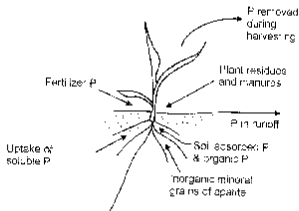
Figure 2.5 Generalized phosphorus gains and losses in the rock-soil plant system (Source: Adapted from van Straaten, 2007).
