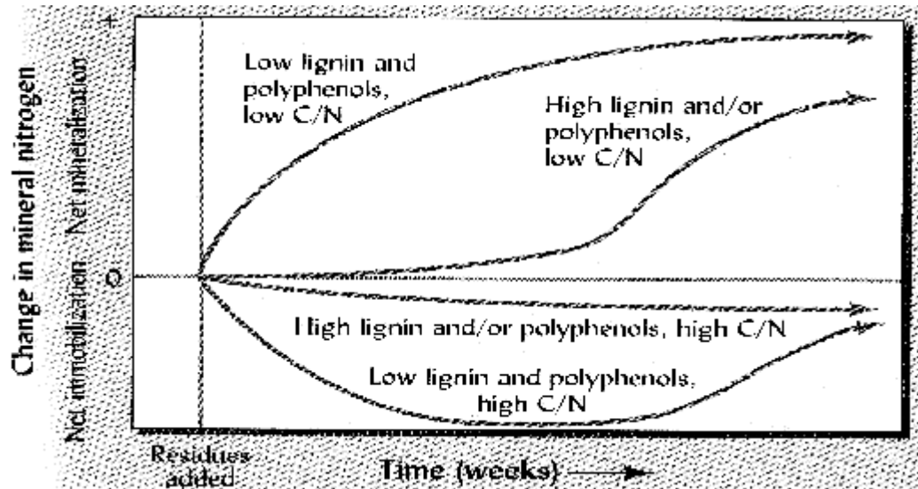
Figure 2.2 Temporal patterns of nitrogen mineralization or immobilization with organic residues differing in C/N ratios and contents of lignin and polyphenols. 2
