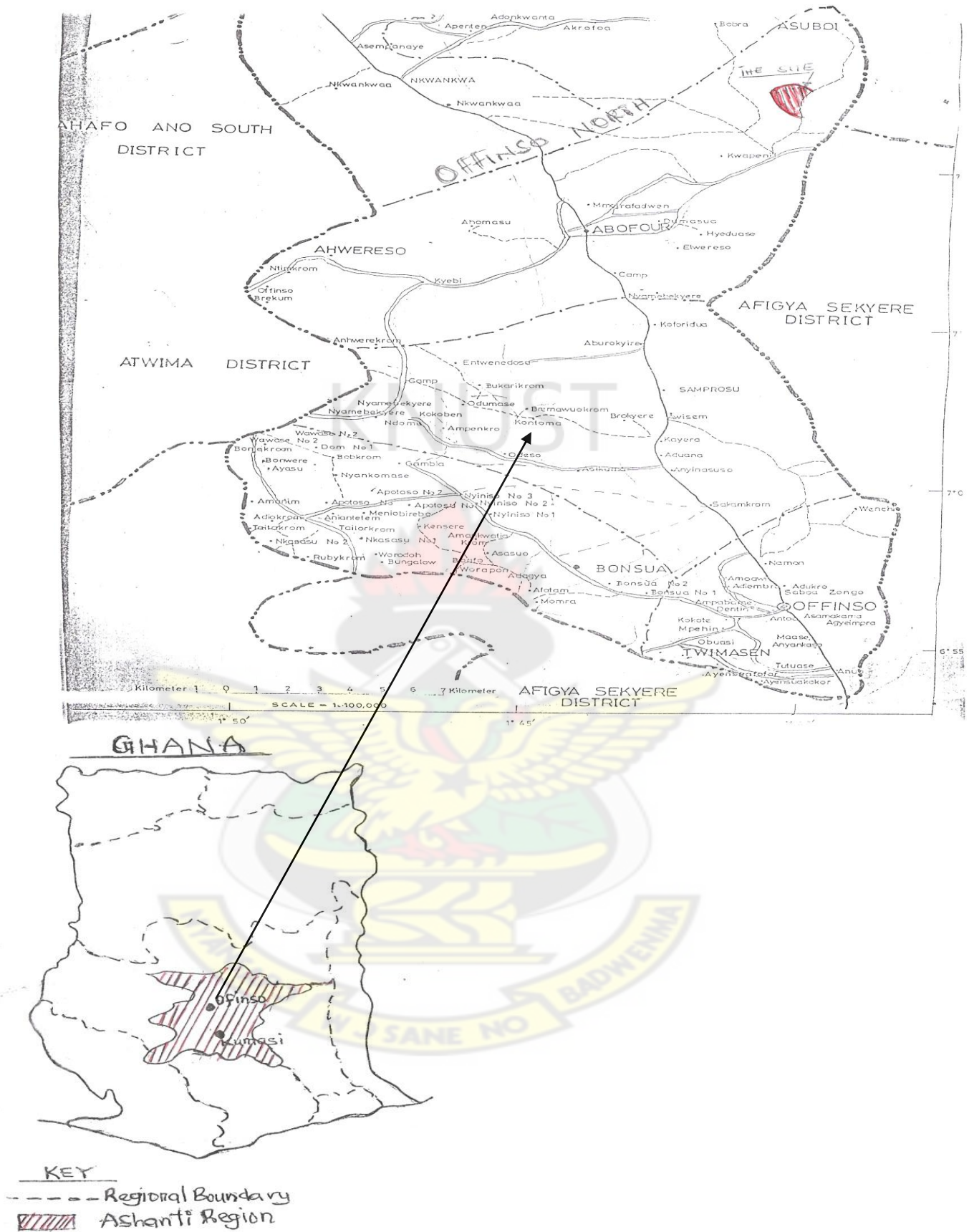
Fig.1: Maps of Study site; Ghana map showing regional boundaries with region where study was conducted highlighted
