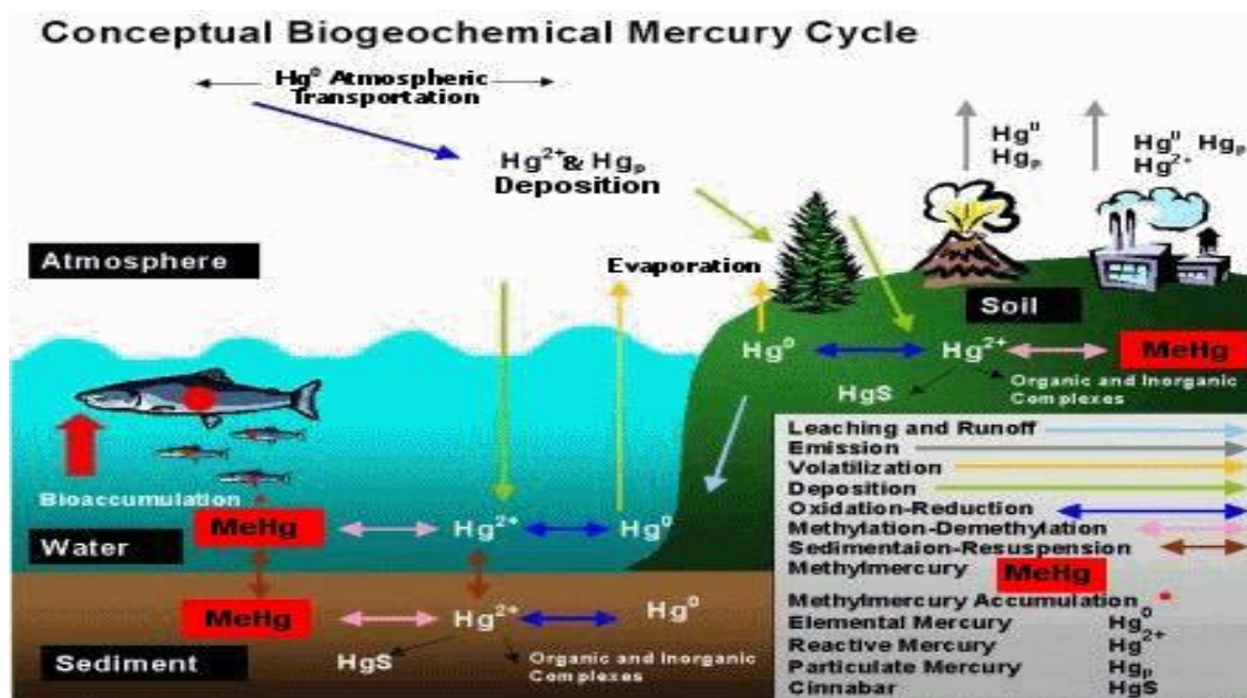
Figure 2.2: The Biochemical cycle of Mercury
