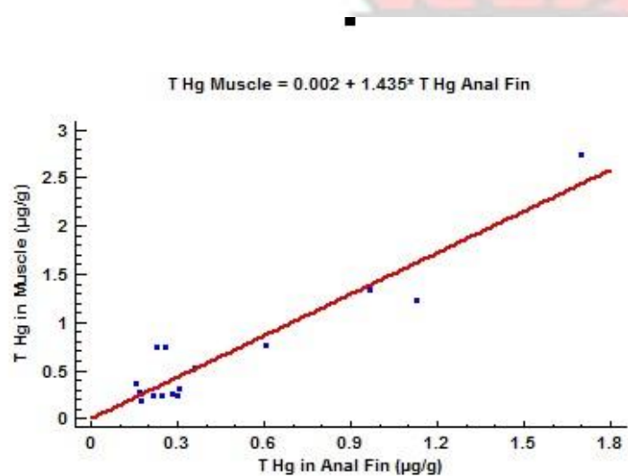
Figure 4.35: T Hg in Muscles Verses T Hg in Anal fins of Tilapia fish from Yapei
