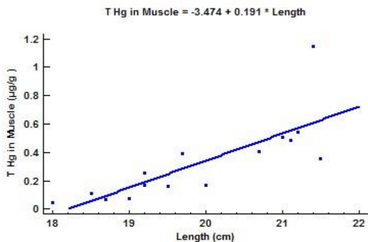
Figure 5.8: T Hg in Muscle versus Length
