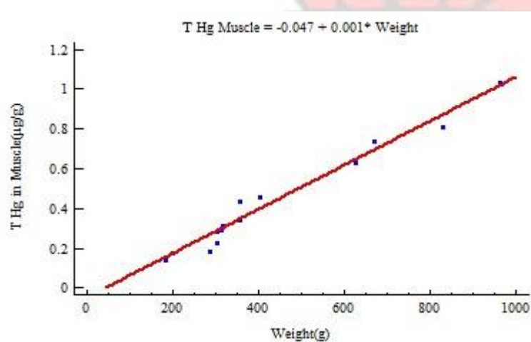
Figure 4.47: T Hg in Muscle Verses Weight
