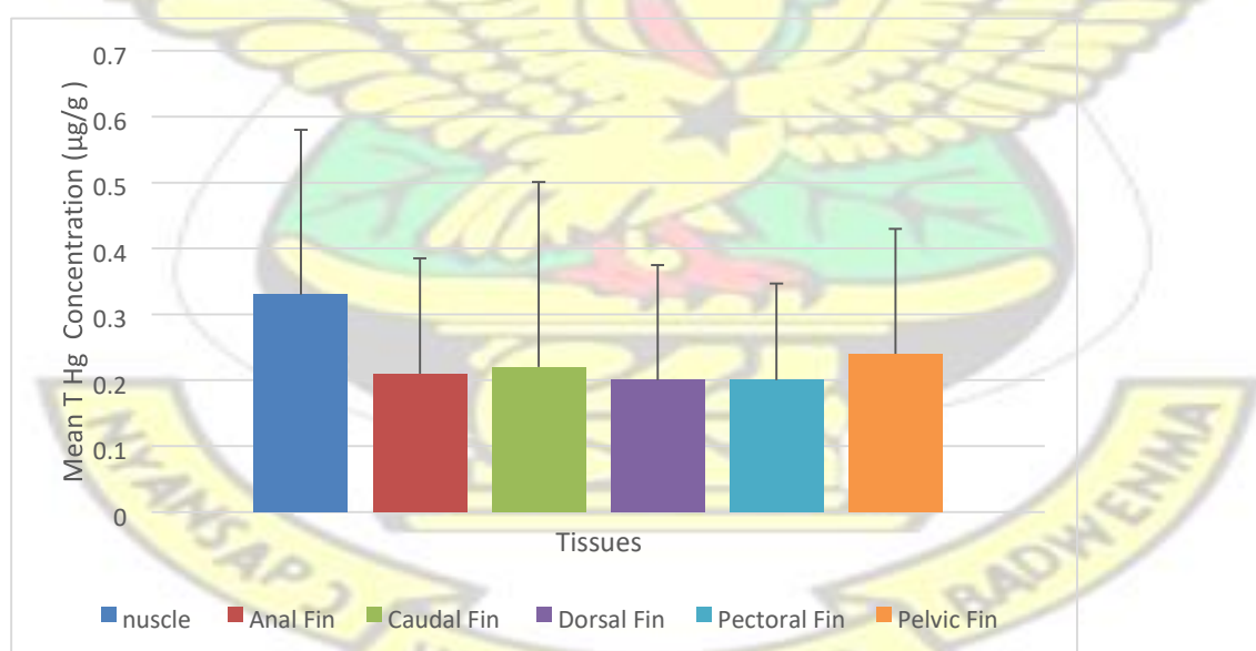
Figure 4.1: Results for Mean Mercury in Muscle tissue and various fins for Tilapia Sample
