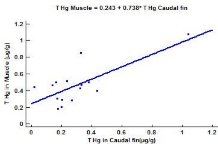
Figure 4.10: T Hg in Muscles Verses T Hg in Caudal fins
