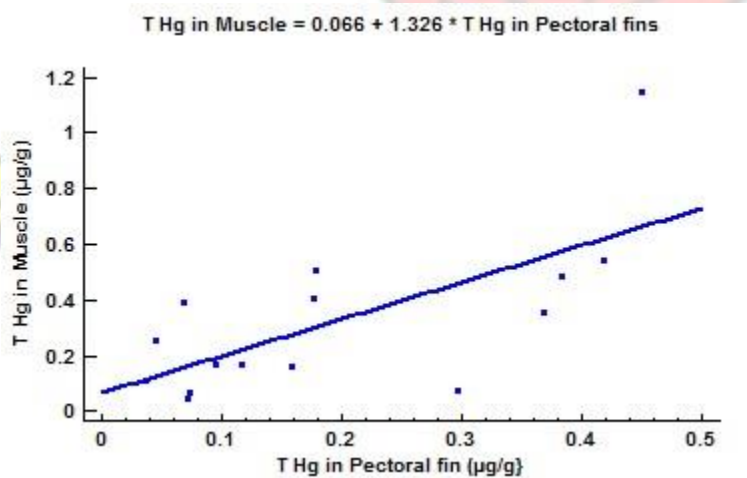
Figure 5.4: T Hg in Muscle verse T Hg in Pectoral fins
