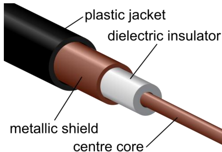
Figure 2.4 Coaxial cable cutaway
