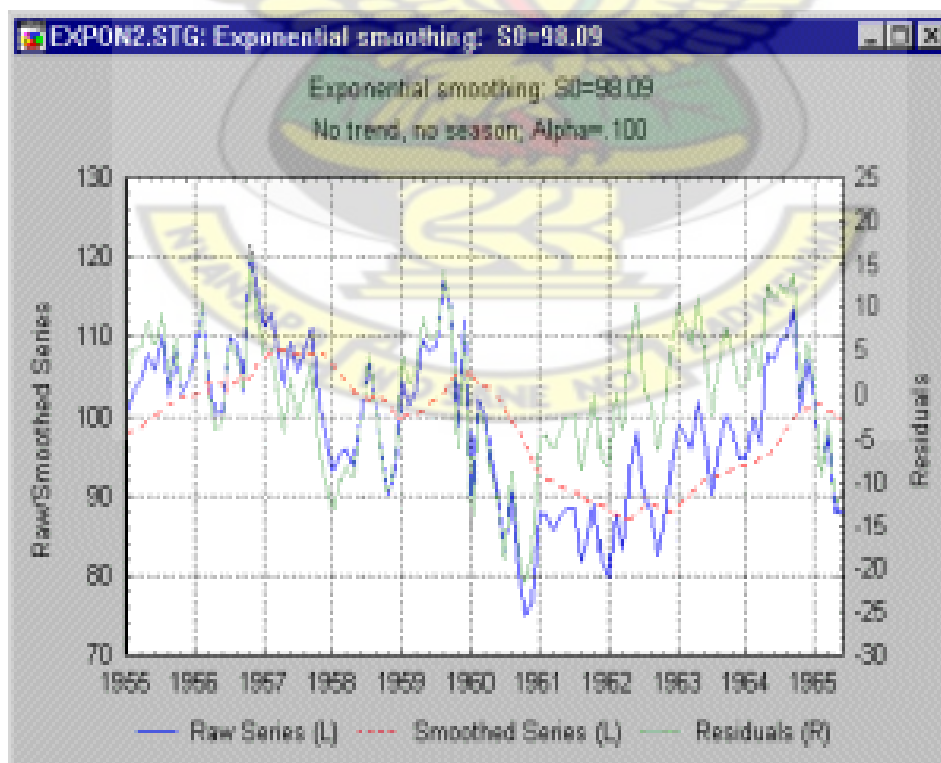
Figure 3.5: Graph of Exponential smoothing
